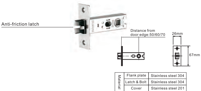
Single latch
