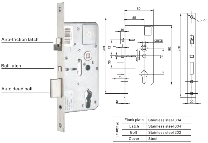
Mortise European 3#
