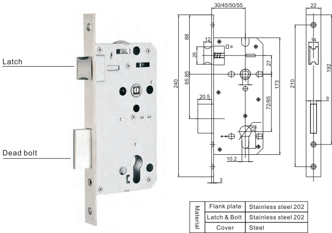
Mortise European(3072/85,4072/85, 4572/85,5072/85,5572/85,6072/85)
