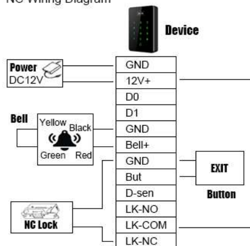
NC Wiring Diagram
